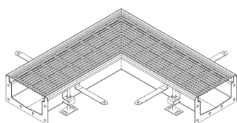
Corner-S2002
