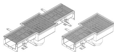
Trash Box-S2004
