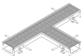
Branch-S2003
