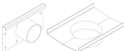
Outlet-S2006
